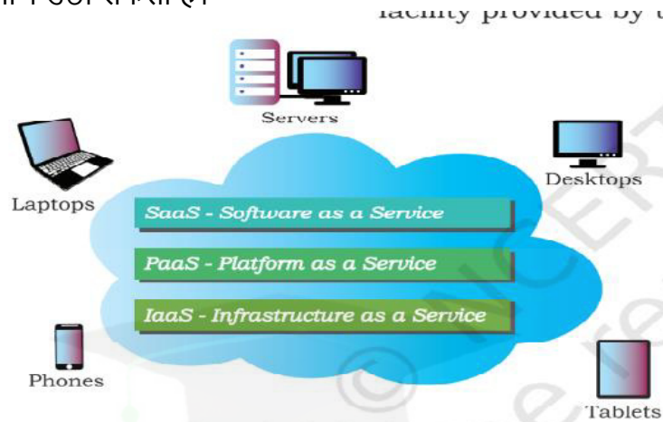
Figure 3.12: Cloud computing
